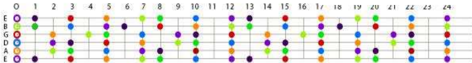
One Octave
